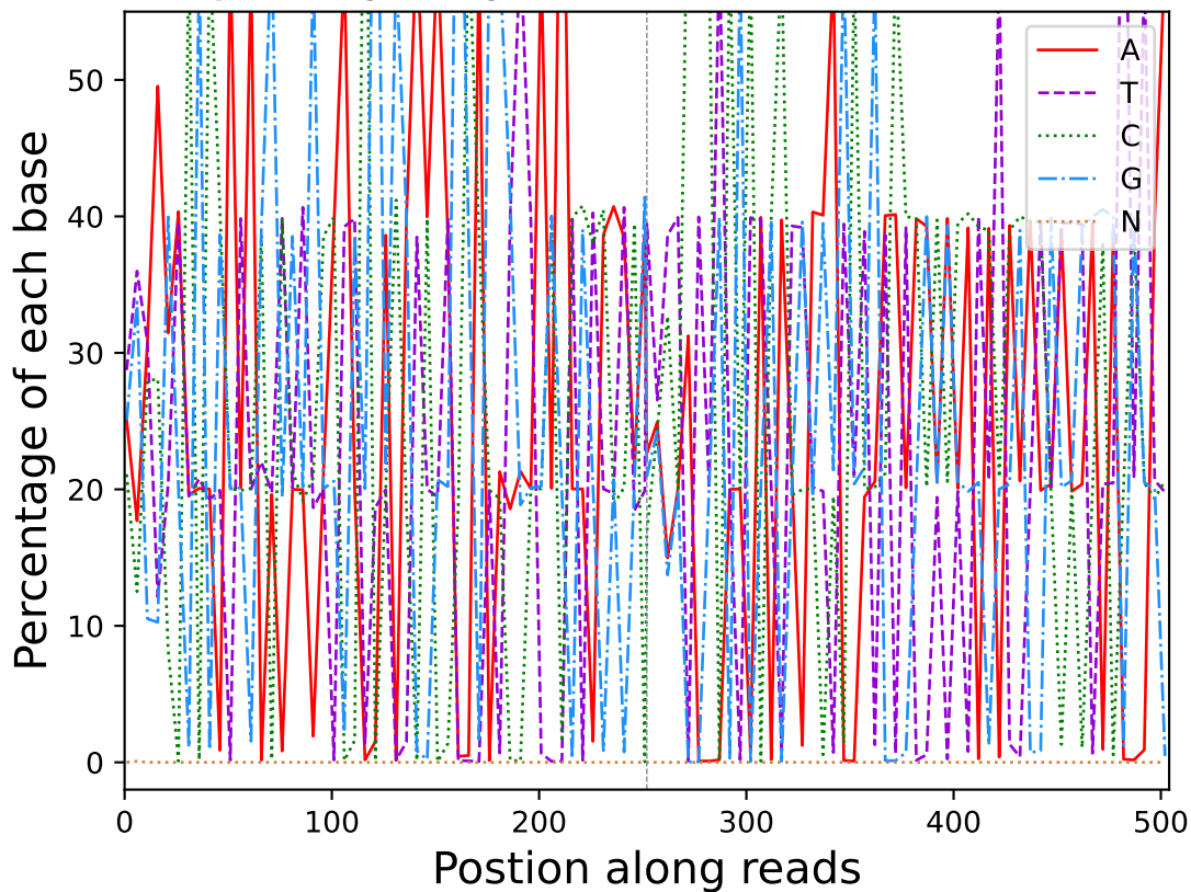
Base percentage along reads (R20218)
